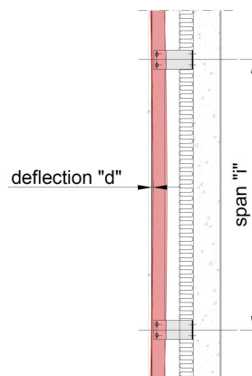
Image 7 – The maximum deflection of the battens/profiles between two brackets d_{max} must be \leq 1/200 for the SrIn between the brackets "i"
