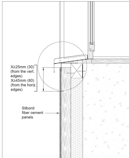
Image 30 – Example of vertical section of a ventilated facade along a window. Wooden subframe.
