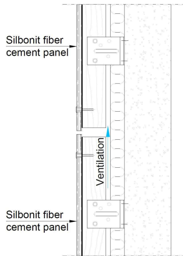
Image 27 – Example of a vertical section of the ventilated facade package along a horizontal joint between panels. Wooden subframe and Silbonit fiber-cement flat-panel cladding.
