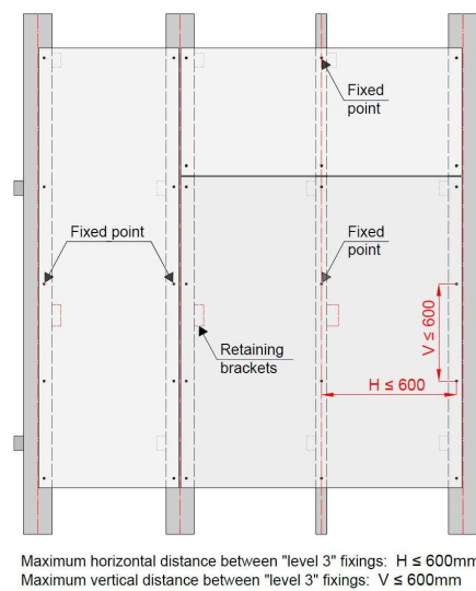
Image 18 – Example of cladding with Silbonit fiber-cement panels. The retaining bracket shown in red should be as close as possible to the fixed point of the panel.
