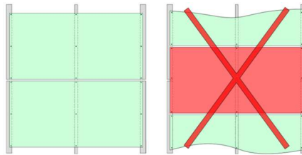
Image 23 – Left: example of a correct way to secure Silbonit panels, with the horizontal joint of the cladding aligning with the expansion joint of the subframe profiles. Right: example of an incorrect way to secure the Silbonit panels, with a cladding sheet secured to two profiles.
