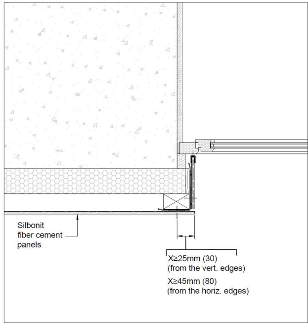
Image 32 – Example of horizontal section of a ventilated facade along a window. Wooden subframe.
