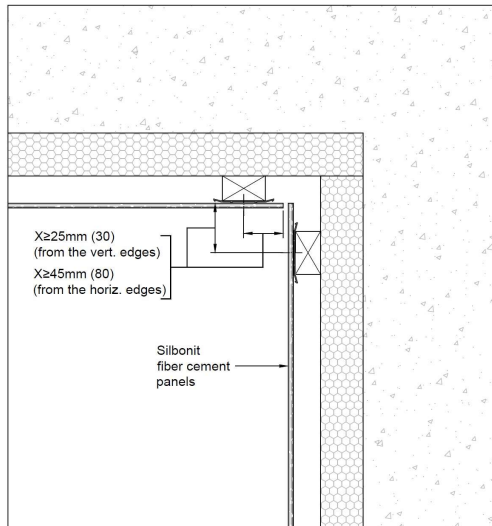
Image 28 – Example of a horizontal section of the ventilated facade package along an inner corner with an open vertical joint between the cladding panels. Wooden subframe.
