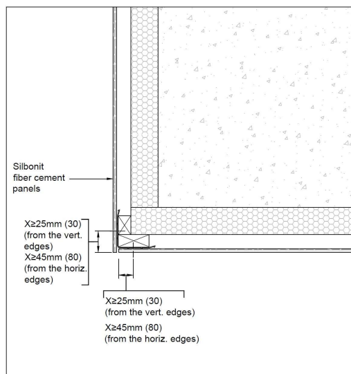
Image 29 – Example of a horizontal section of the ventilated facade package along an external corner with an open vertical joint between the cladding panels. Wooden subframe.
