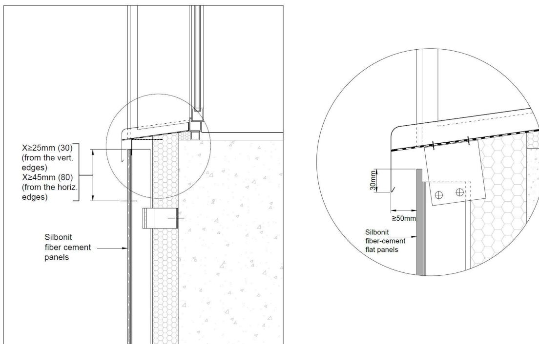
Image 35 – Example of vertical section of a ventilated facade along a window. Aluminum subframe.
