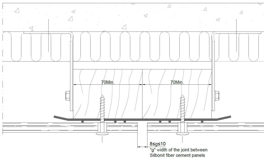
Image 26 – Example of a horizontal section of the ventilated facade package along a vertical joint between panels. Note the protective gasket and the minimum width of the wooden battens.
