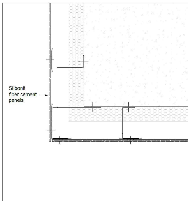
Image 37 – Example of a horizontal section of the ventilated facade package along an external corner with an open vertical joint between the cladding panels. Aluminum subframe.
