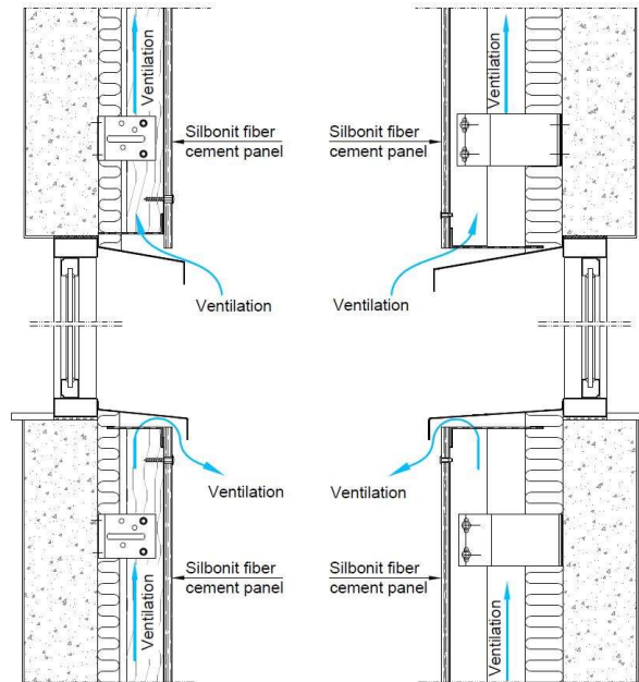
Image 25 – Example of a section of a ventilated facade package along a window. Wooden subframe on the left and aluminum subframe on the right, both cladded with Silbonit fiber-cement flat panels
