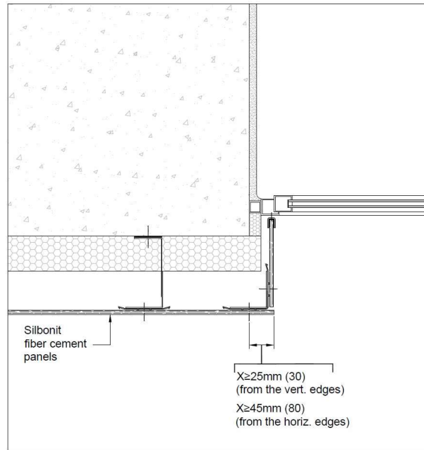
Image 36 – Example of horizontal section of a ventilated facade along a window. Aluminum subframe.
