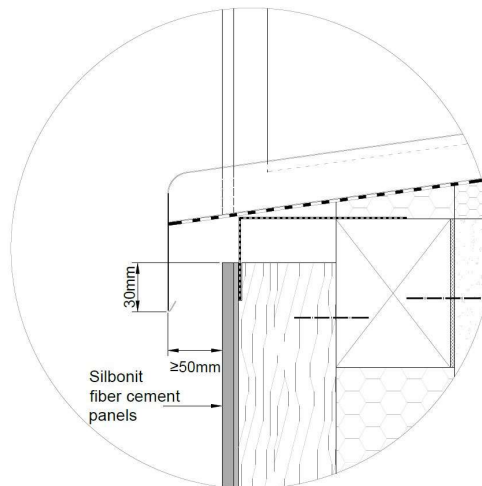
Image 31 – Example of vertical section of a detail of the cladding beneath a window.
