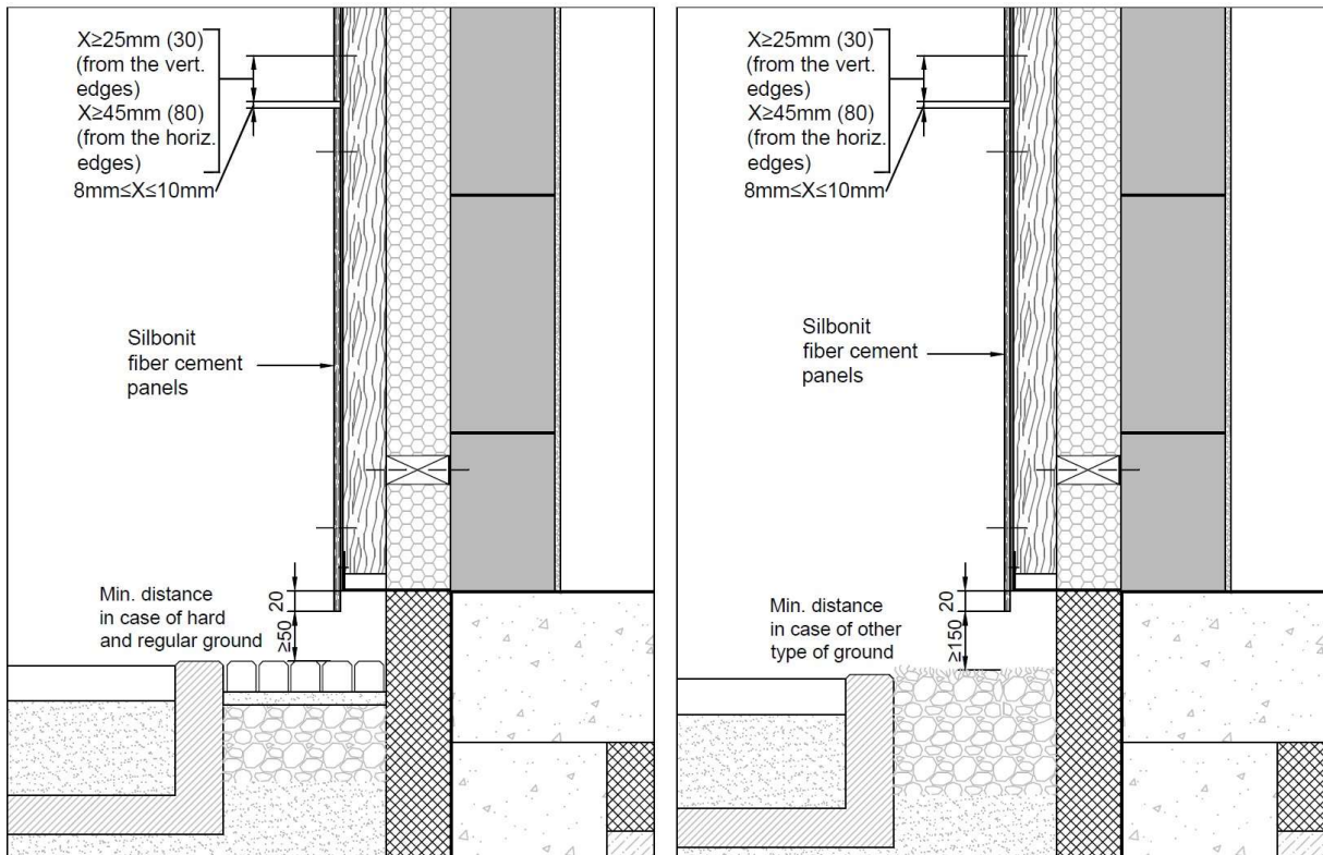
Image 33 – Example of vertical sections of the base of the ventilated facade cladding with two different slab solutions at the base of the building. Wooden subframe.
