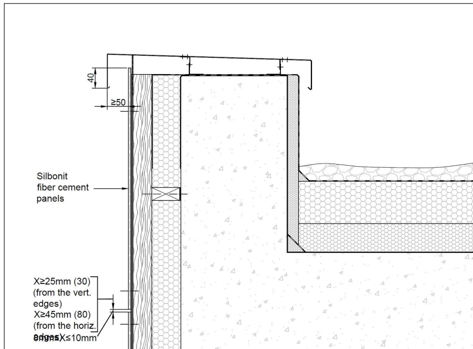
Image 34 – Example of vertical sections of the coping of the ventilated facade cladding. Wooden subframe.
