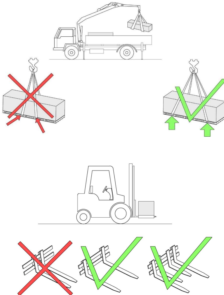
Image 40– Transport and handling of panels
