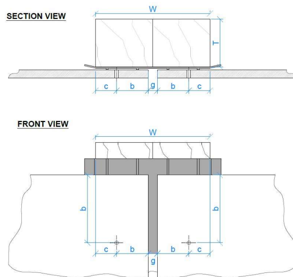
Image 11 – Geometrical specifications of the cladding required to determine the width of the wooden beams of the subframe
