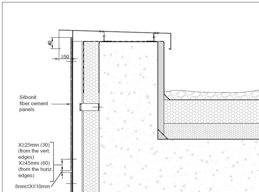
Image 39- Example of a vertical section of the coping of the ventilated facade cladding. Aluminum subframe.
