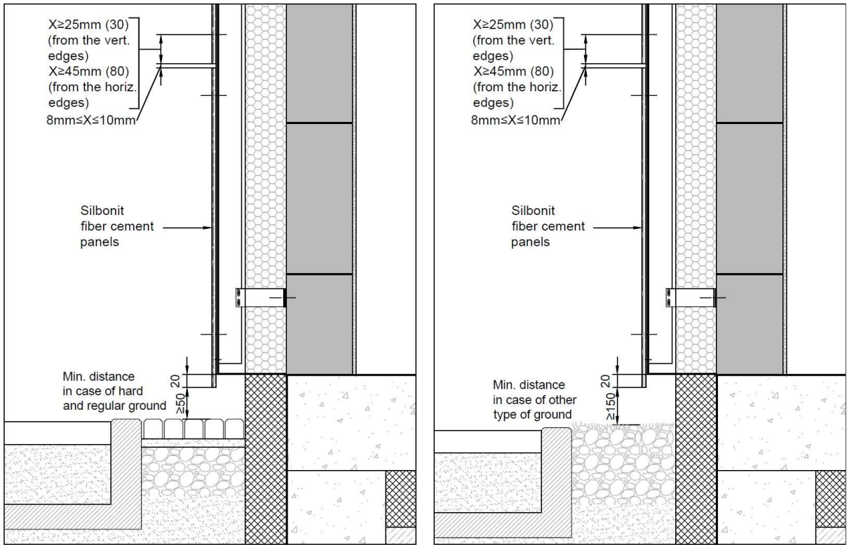
Image 38 – Example of vertical sections of the base of the ventilated facade cladding with two different slab solutions at the base of the building. Aluminum subframe.
